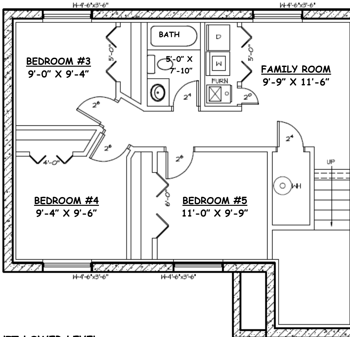
5 BEDROOM UNIT LOWER LEVEL
